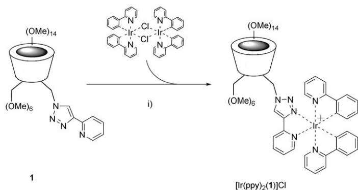
Scheme 3. Synthesis of [Ir(ppy) 2 ( 1 )]Cl. Conditions: i) chloroform/methanol, 3:1 (v/v), 45 °C, 3 h.
