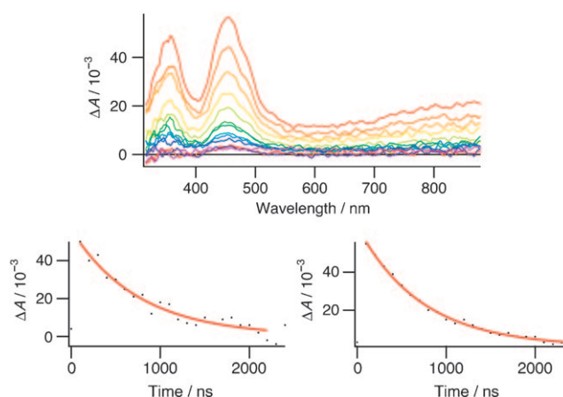
Figure 4. Top: Transient absorption spectrum of [Ir(ppy) 2 ](1)Cl after laser light excitation at \lambda = 380 nm, with decay kinetics at \lambda = 360 nm (bottom left) and \lambda = 449 nm (bottom right). 250 accumulations per frame, 25 frames (only first and odd numbered frames are shown in the transient spectrum for clarity), 100 ns increment in between frames. Decay at \lambda = 360 nm, \tau = 754 ns. Decay at \lambda = 449 nm, \tau = 723 ns.
