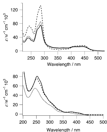
Figure 1. UV/Vis absorption spectra of Ru complexes (top; —, [Ru(bpy) 2 ( 1 )]Cl 2 ; ·····, [Ru(bpy) 2 ( 2 )]Cl 2 ; ----, [Ru(bpy) 2 ( 3 )]Cl 2 ) and Ir complexes (bottom; —, [Ir(ppy) 2 ( 2 )]Cl; ----, [Ir(ppy) 2 ( 1 )]Cl; ·····, [Ir(F 2 ppy) 2 ( 2 )]Cl) in water.
