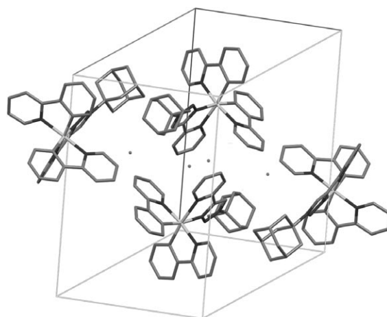
Figure 5. Unit cell of [\text{Ir}(\text{ppy})_2(\mathbf{2})]\text{Cl} . The top and bottom structures toward the left are \Delta ; the top and bottom ones toward the right are \Lambda . Hydrogen atoms and solvent ( \text{H}_2\text{O} ) molecules are omitted for clarity.
