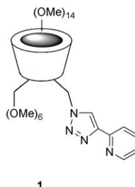
Scheme 1. Preparation of pytl by the Cu-catalyzed Huisgen dipolar [3+2] cycloaddition.
