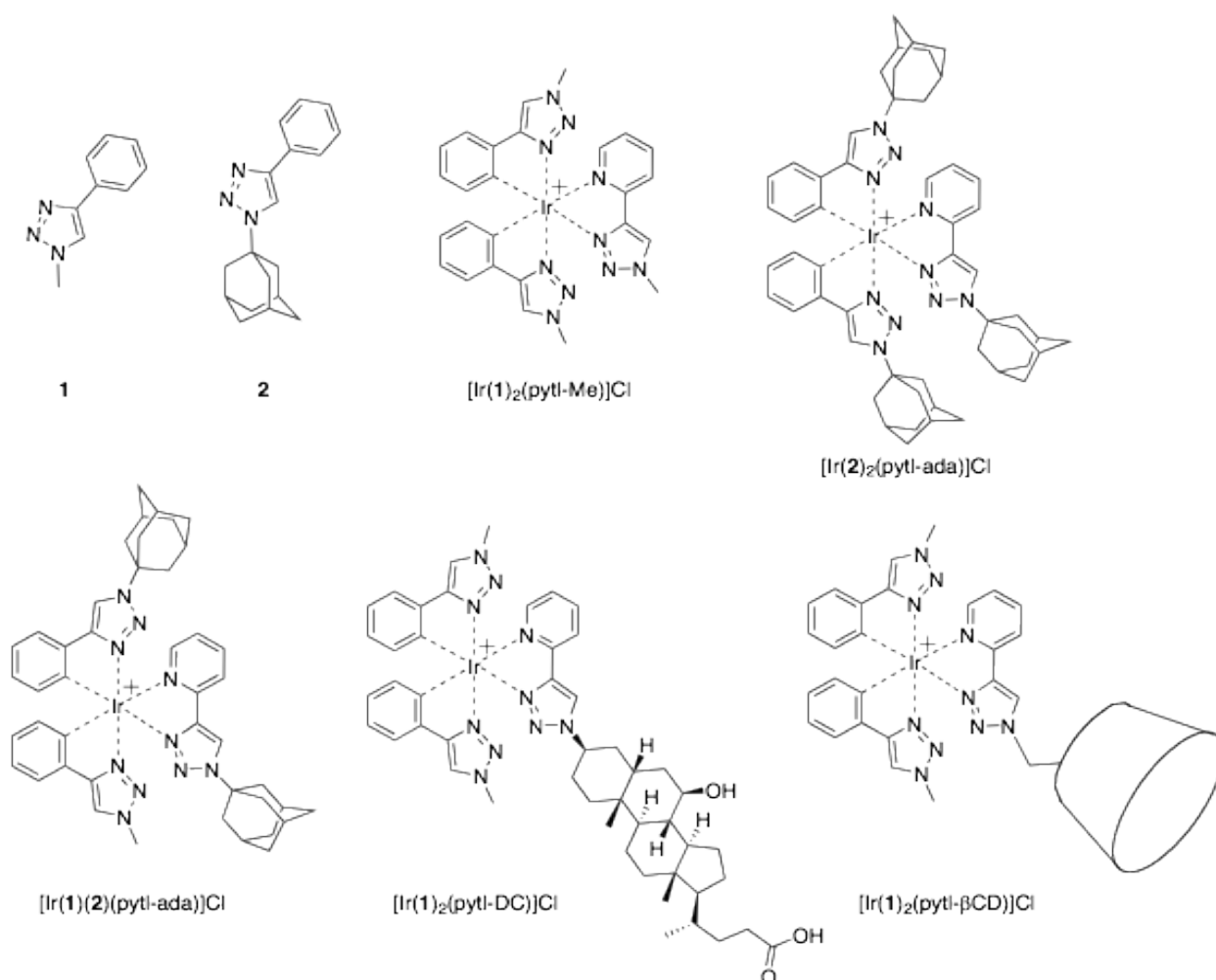
Scheme 1. Structures of phtl-me 1 , phtl-ada 2 and their heteroleptic iridium complexes.
