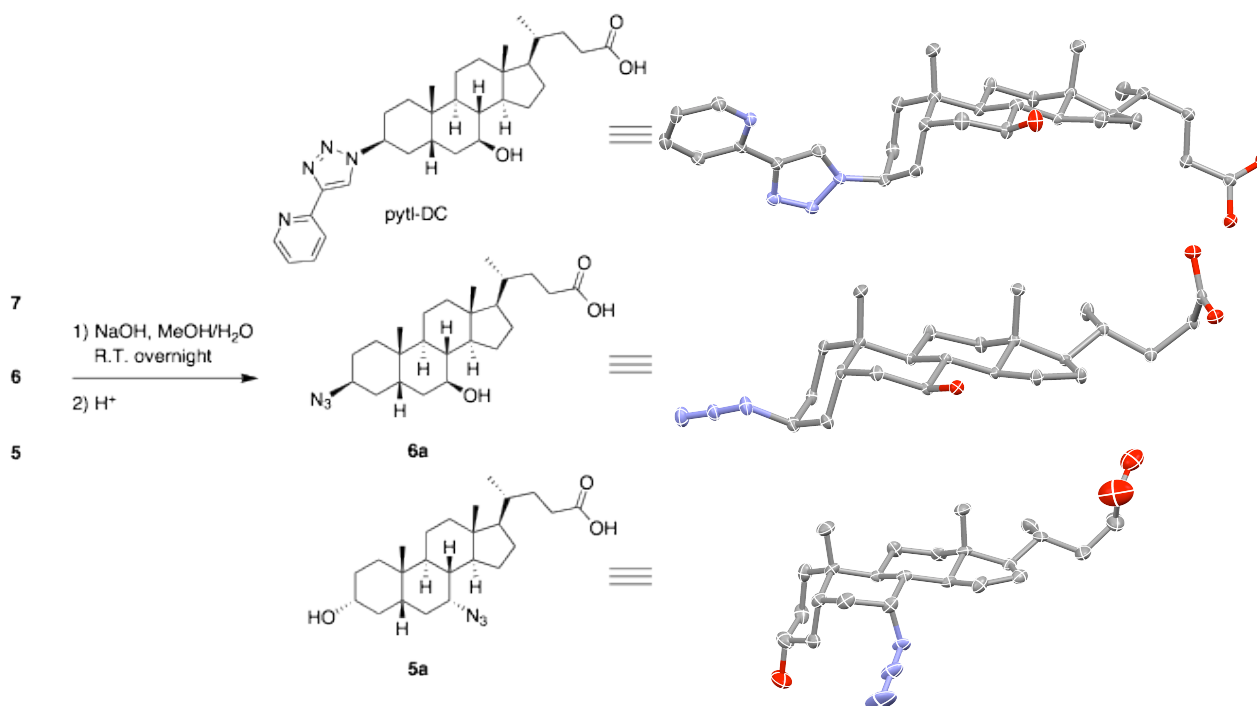
Scheme 4. Preparation and crystal structures of pytl-DC, 5a and 6a . Gray, carbon; blue, nitrogen; red, oxygen. The thermal ellipsoids for the image represent 25% probability limit. Hydrogen atoms are omitted for clarity.
