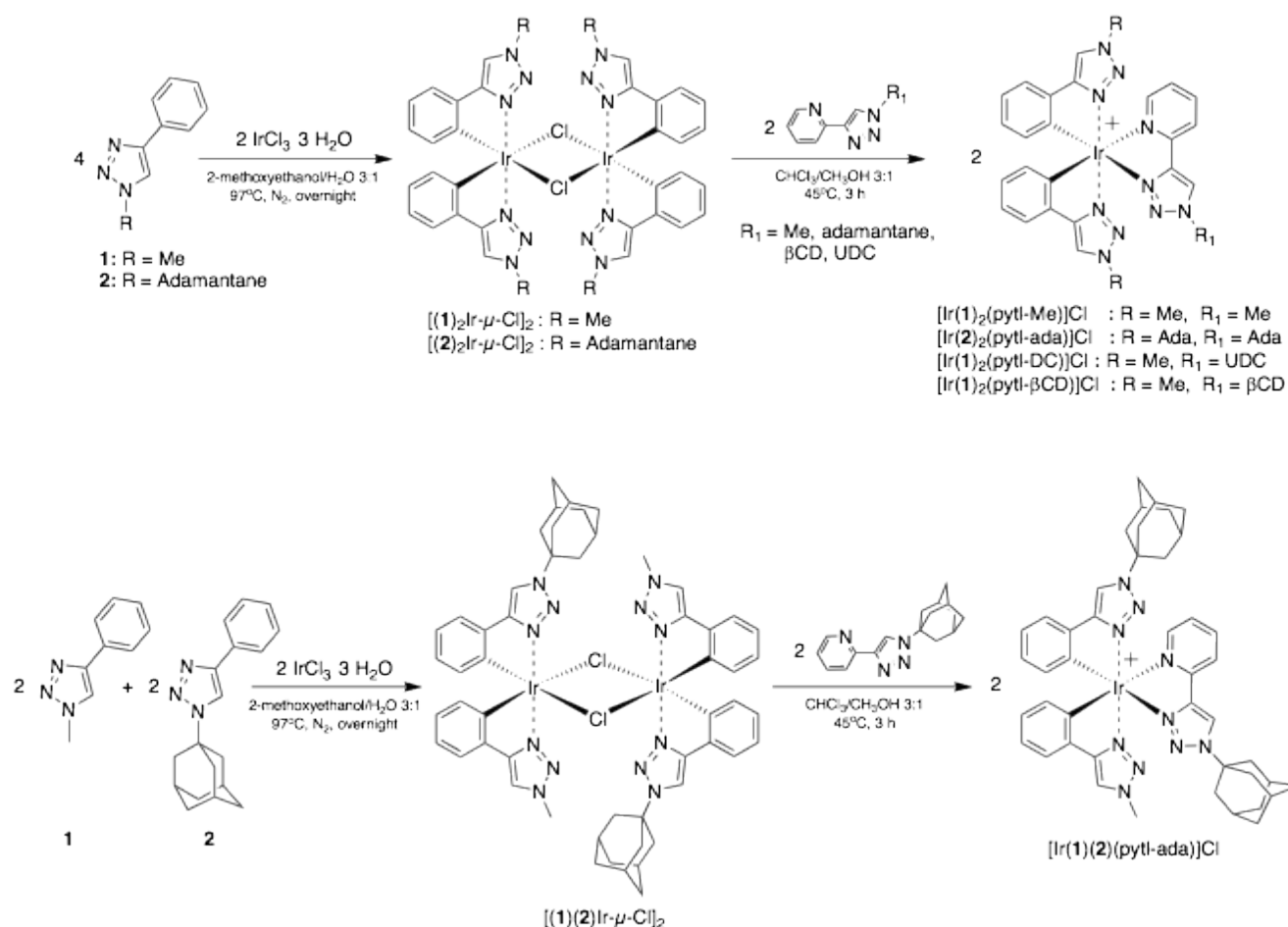
Scheme 5. Synthesis of the iridium III complexes.
