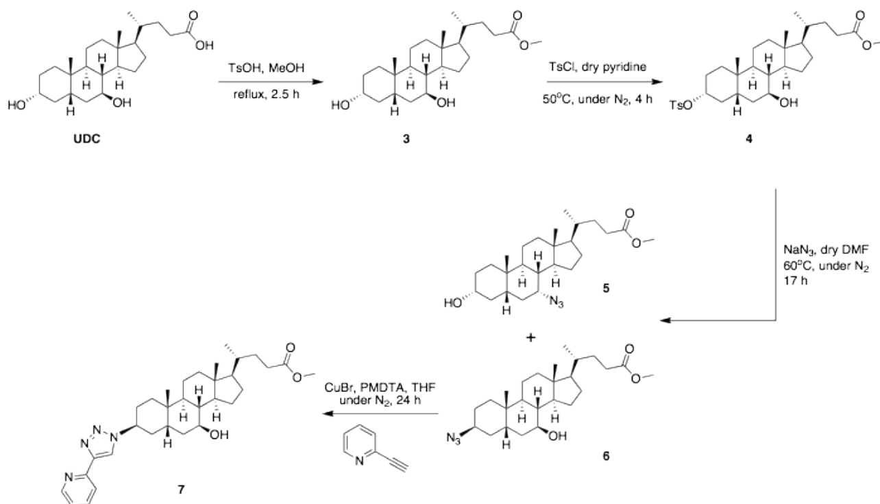
Scheme 3. Synthesis of 7 .
